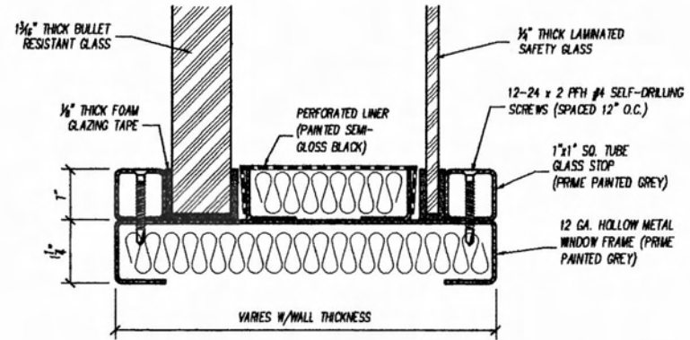
QUIETLITE - BULLET-RESISTANT WINDOW
