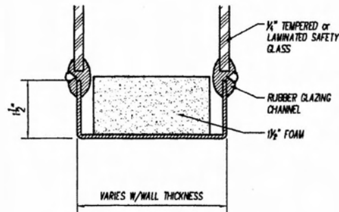
QUIETLITE - 'U' FRAME WINDOW
