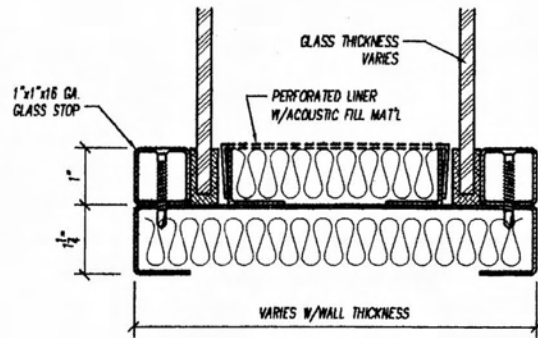
QUIETLITE - 'HM' WINDOW
