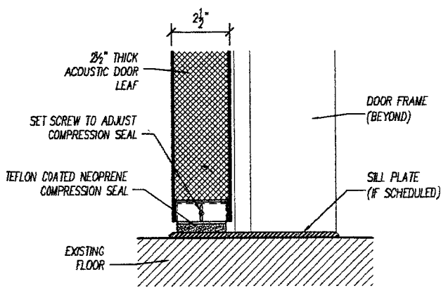
SILL DETAIL
