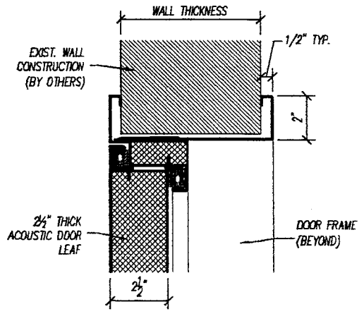
HEAD DETAIL
